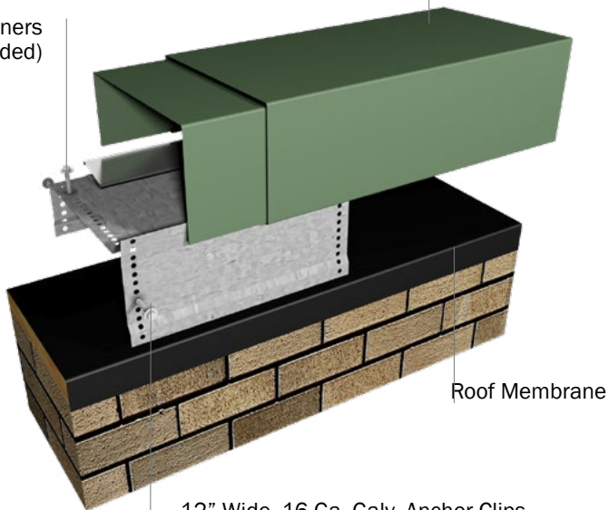
12" Wide, 16 Ga. Galv. Anchor Clips (Spacing Determined by Manufacturer)
